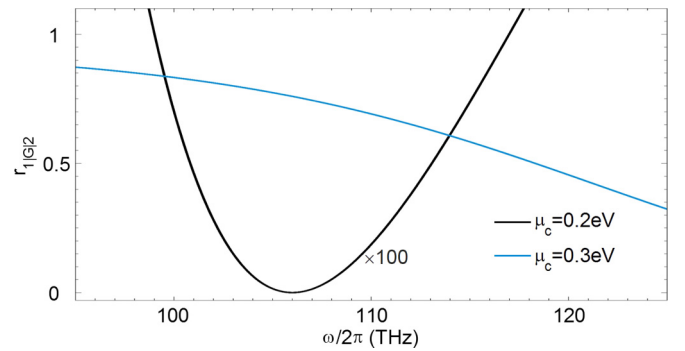
FIG. 10. Tunable TE wave reflectance from monolayer graphene through varying the chemical potential. The propagating TE wave is incident from region 1 with an incident angle of 89.1^\circ . The other parameters are the same as those in Fig. 9. For the purpose of clear demonstration, the black line is multiplied by a factor of 100. Since the chemical potential in graphene can be flexibly tunable through the electrostatic gating, it is advantageous to use graphene to design tunable optical devices. The negligible reflectance ( \{<\}1\% ) over the broad frequency range (99–117 THz) would become significant ( >50\% ) when tuning the chemical potential of graphene from 0.2 to 0.3 eV. This suggests that graphene might be used as a real-time tunable ultrathin antireflection coating.
