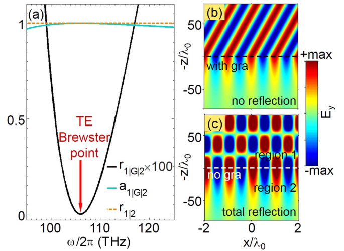
FIG. 9. Infrared nonmagnetic TE Brewster effect created by using monolayer of graphene under oblique incidence at 106 THz. The reference wavelength is \lambda_0 = 2.83 \mu\text{m} . The relative permittivities in nonmagnetic regions 1 and 2 are \epsilon_{1r} = 1.00028 and \epsilon_{2r} = 1 , respectively. We set the chemical potential \mu_c = 0.2 eV, the temperature T = 300 K, and the relaxation time \tau = 0.1 ps in graphene. (a) Spectra of reflectance and absorbance. The value of r_{1|G|2} is multiplied by a factor of 100. (b–c) Total electric field in each region with (b) and without (c) graphene at the dielectric interface. The propagating TE wave is incident from region 1 with an incident angle of 89.1^\circ . For a clear demonstration, the scale on the y axis is compressed in (b,c), compared with that of the x axis. Note that the curves in Fig. 9(a) are the same as the curves in Fig. 3(a). This is because when satisfying the nonmagnetic TE Brewster conditions of Eqs. (5) and (6) in the main text, the reflection coefficient of TE waves in Eq. (2) in the main text is only a function of the surface conductivity of monolayer graphene, independent of the graphene’s layer number.
