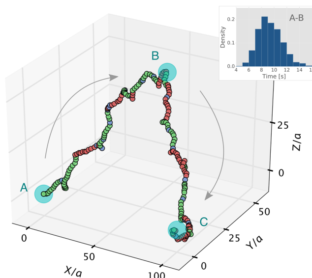
Figure 5. Example of a composite asymmetric particle ( a = 1 \mu\text{m} , Figure 1) transported along the target A–B–C route, by switching the wavelength of the actuating light: 800 nm (red circles) and 500 nm (green circles). At times, the heating is temporarily turned off to allow for rotational diffusion to reorient the particle (blue circles). Inset: histogram of the time required to transport such a particle from A to B ( N = 10^3 runs). See Supporting Information, Video.
