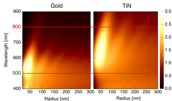
Figure 2. Absorption efficiency as a function of wavelength and radius for a homogeneous gold (left) and titanium-nitride (right) spherical particle, in water. Values obtained from Mie scattering equations. Highlighted green (500 nm) and red (800 nm) lines correspond to the two wavelengths used for selective heating of the two hemispheres of the composite asymmetric particle (Figure 1a).
